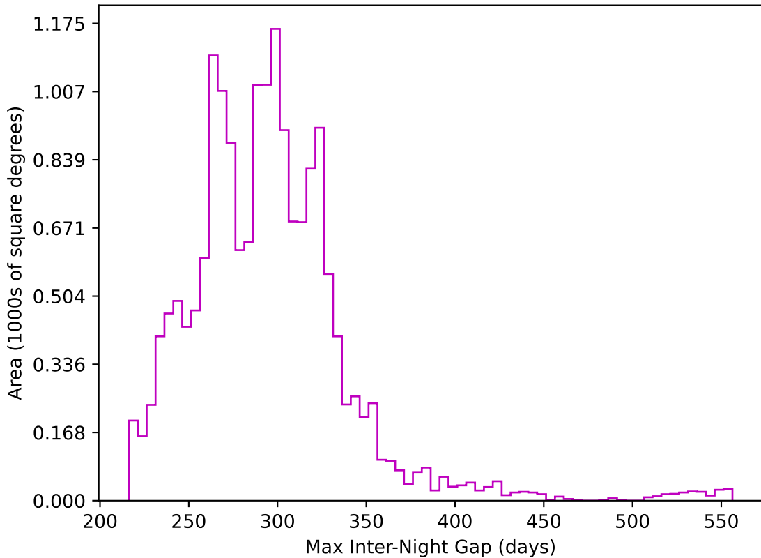
internal_u_expt60_nscale1.1v3.4_10yrs WFD z band: Max Inter-Night Gap
