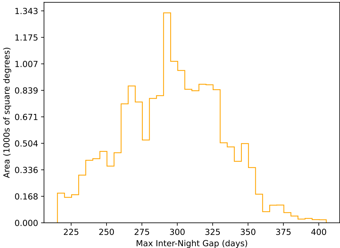
internal_u_expt60_nscale1.1v3.4_10yrs WFD r band: Max Inter-Night Gap
