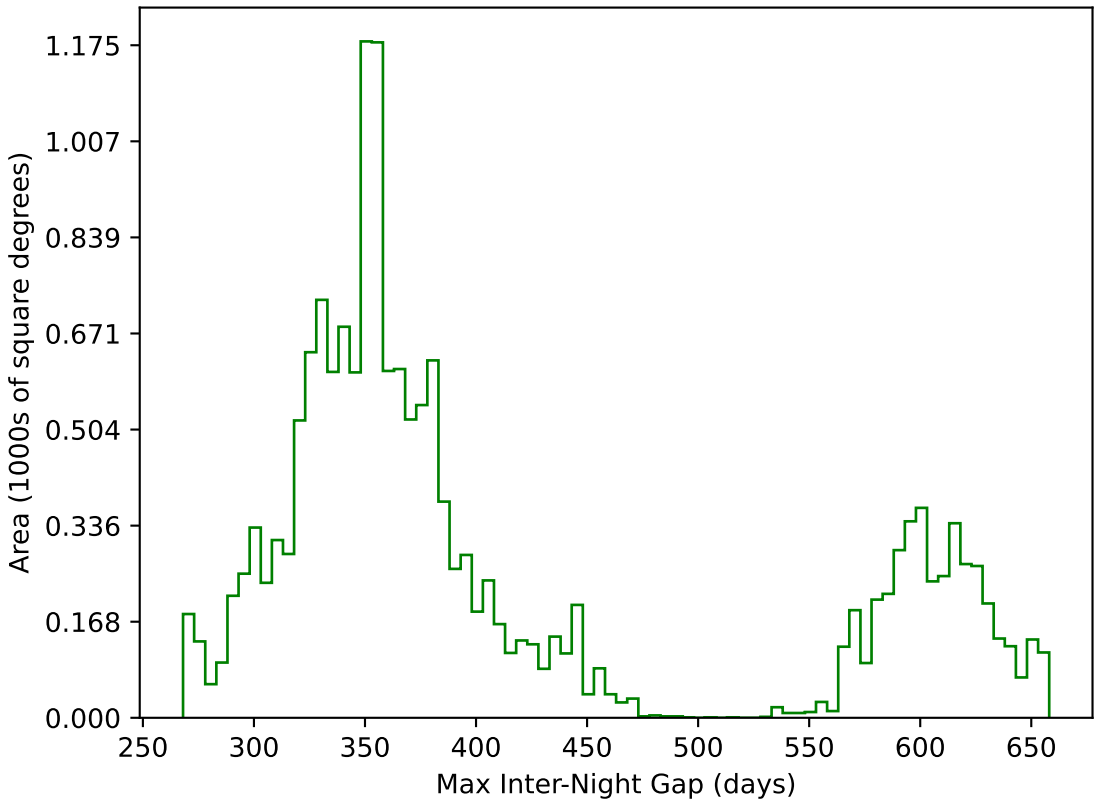
internal_u_expt60_nscale1.1v3.4_10yrs WFD g band: Max Inter-Night Gap
