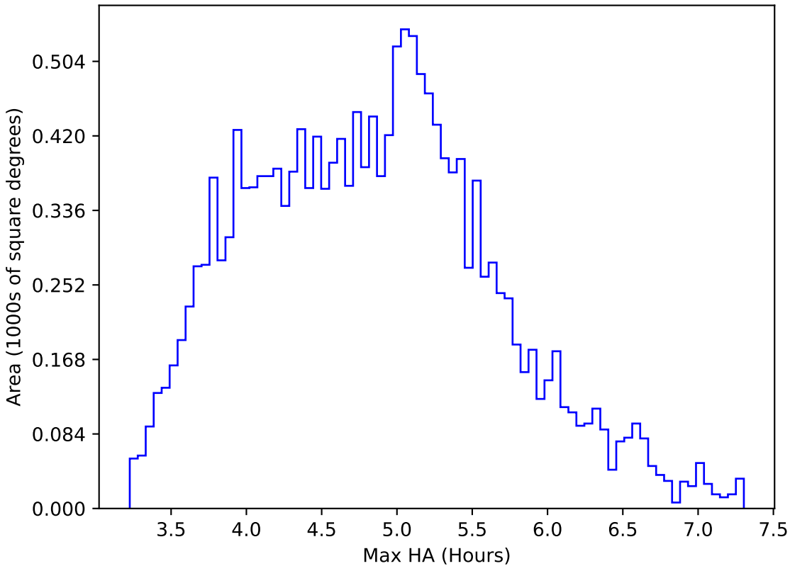
internal_u_expt60_nscale1.1v3.4_10yrs WFD i band: Max HA
