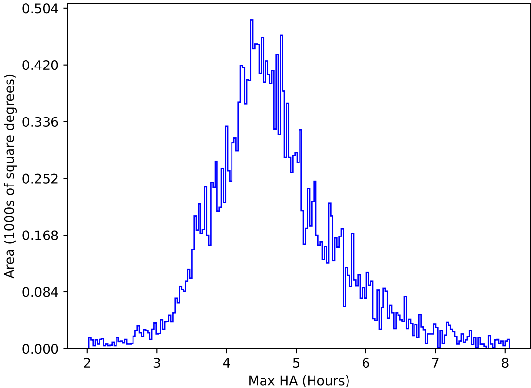
internal_u_expt60_nscale1.1v3.4_10yrs All sky y band: Max HA
