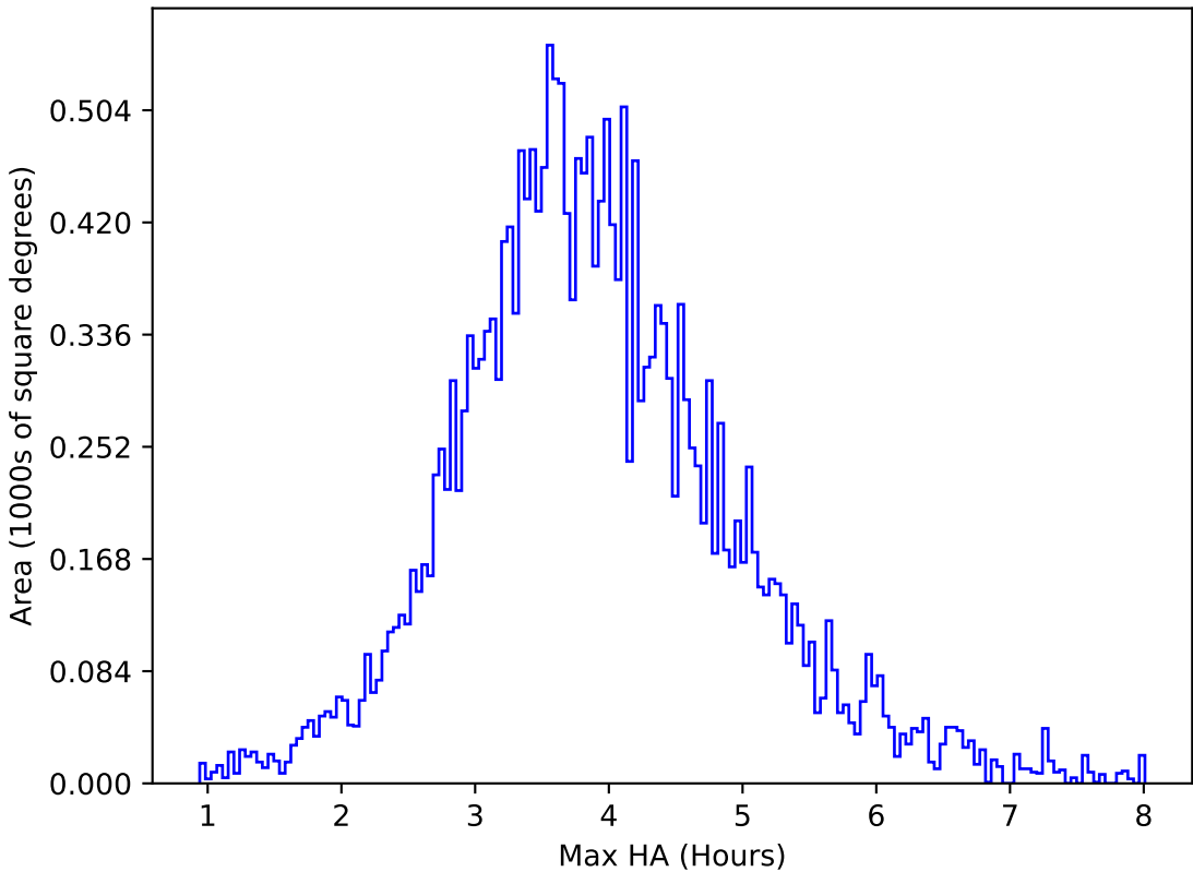
internal_u_expt60_nscale1.1v3.4_10yrs All sky u band: Max HA
