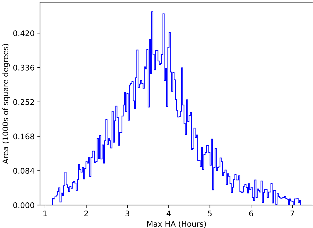
internal_u_expt60_nscale1.1v3.4_10yrs All sky g band: Max HA
