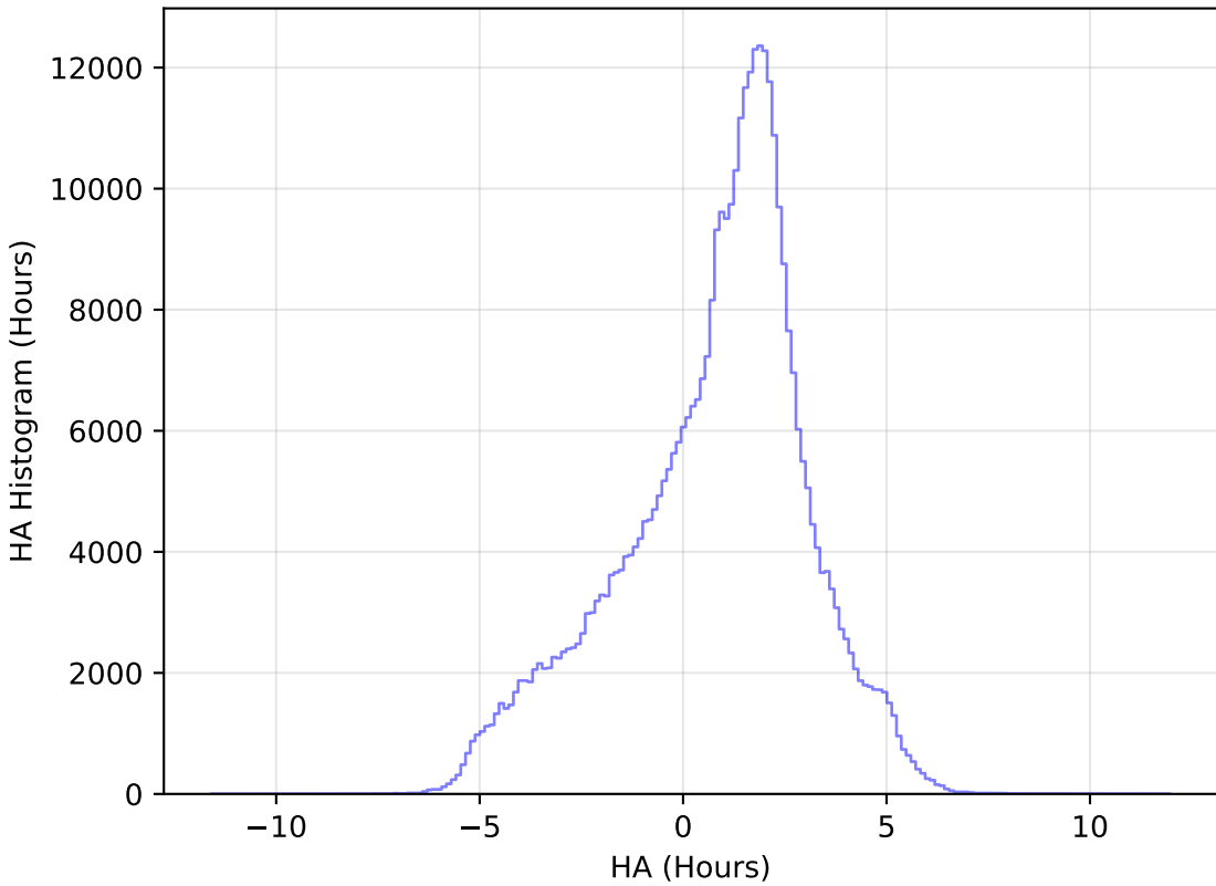
internal_u_expt60_nscale1.1v3.4_10yrs WFD z band: HA Histogram
