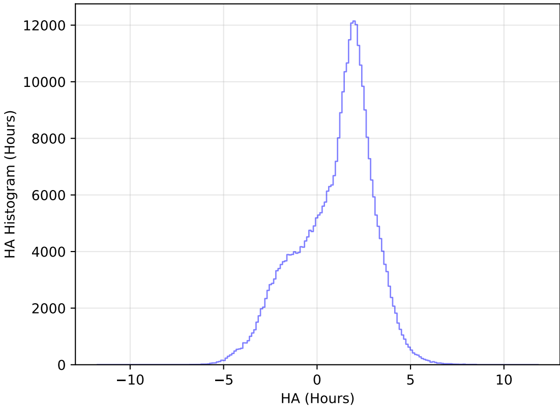
internal_u_expt60_nscale1.1v3.4_10yrs WFD y band: HA Histogram
