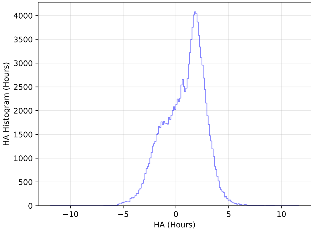
internal_u_expt60_nscale1.1v3.4_10yrs WFD u band: HA Histogram
