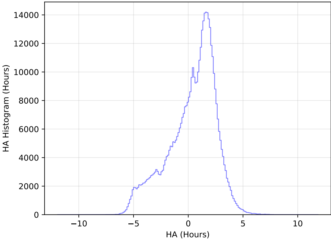
internal_u_expt60_nscale1.1v3.4_10yrs WFD r band: HA Histogram
