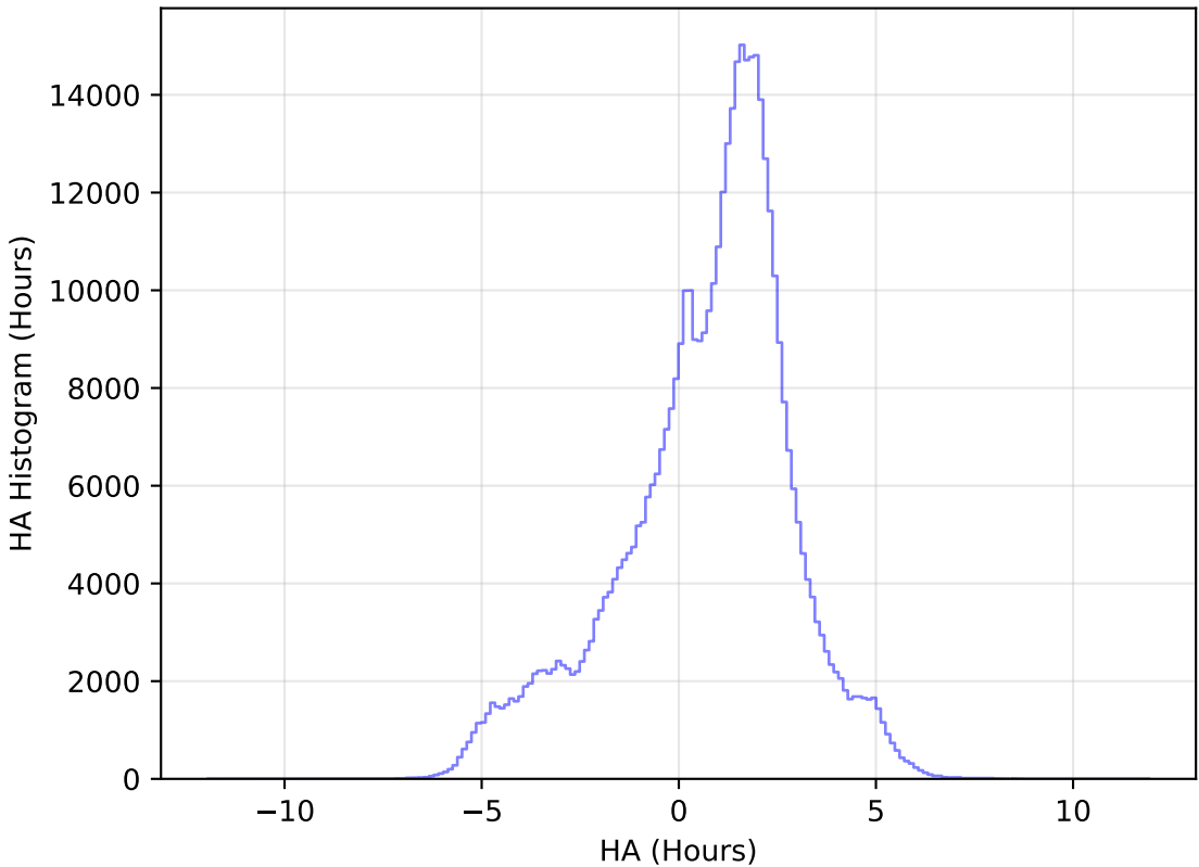
internal_u_expt60_nscale1.1v3.4_10yrs WFD i band: HA Histogram
