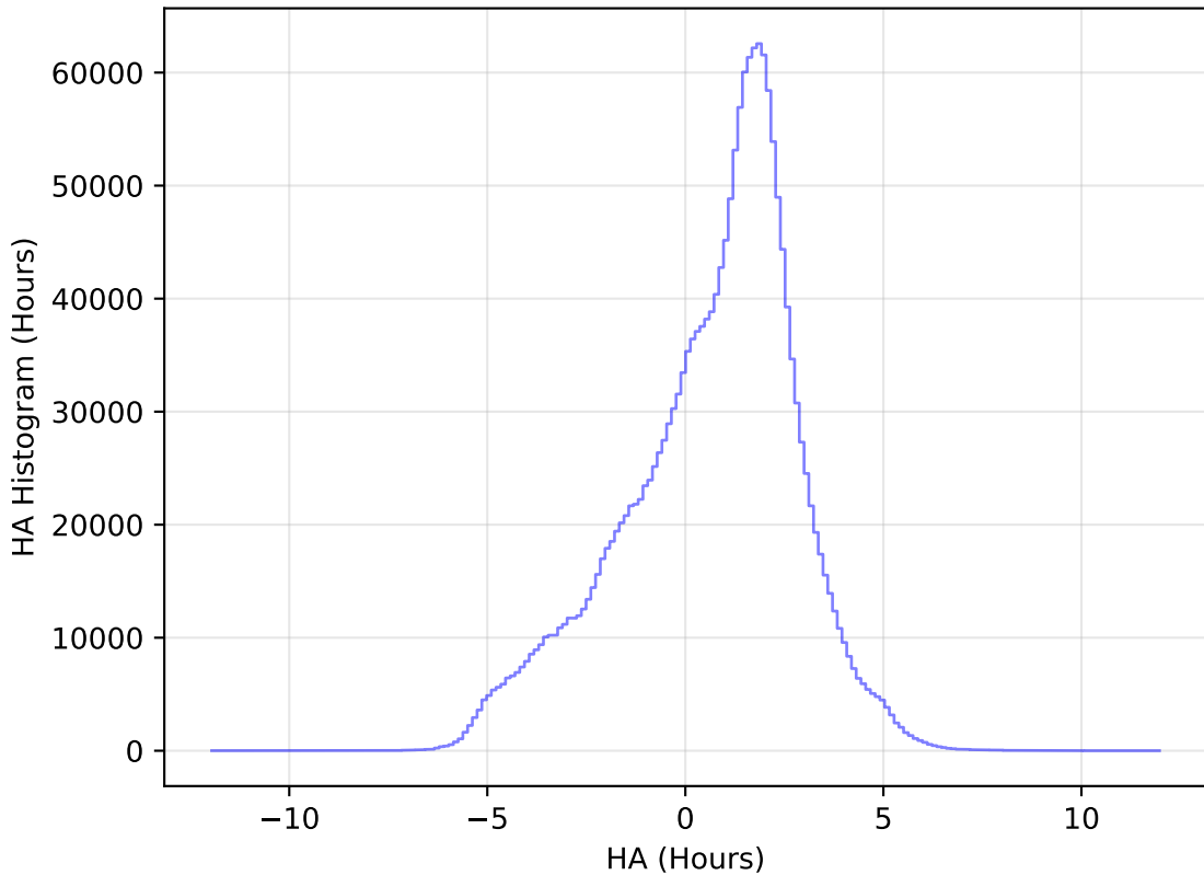
internal_u_expt60_nscale1.1v3.4_10yrs WFD all bands: HA Histogram
