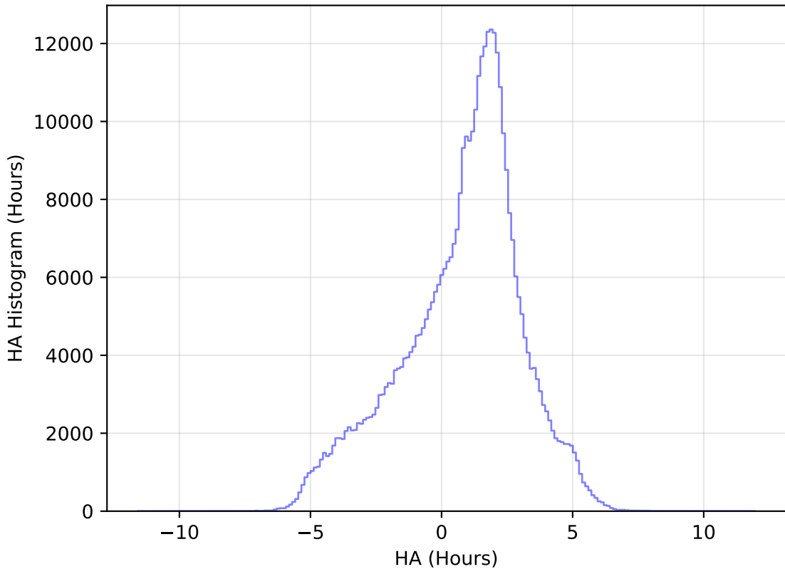
internal_u_expt60_nscale1.1v3.4_10yrs All sky z band: HA Histogram
