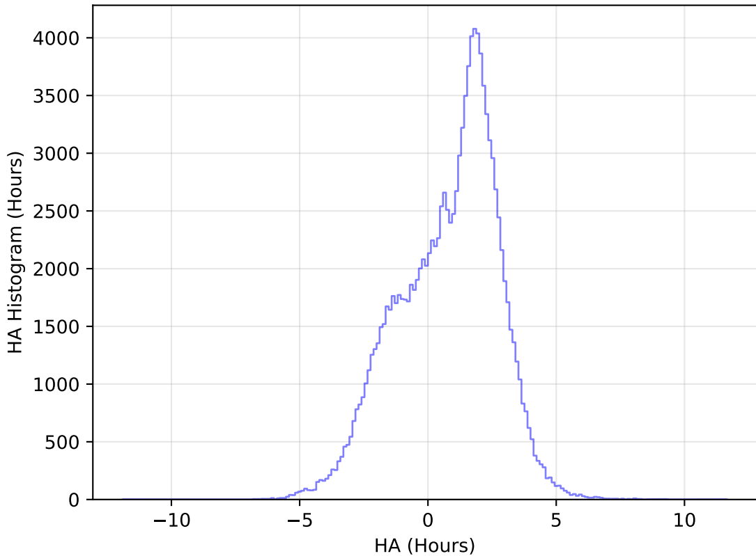
internal_u_expt60_nscale1.1v3.4_10yrs All sky u band: HA Histogram
