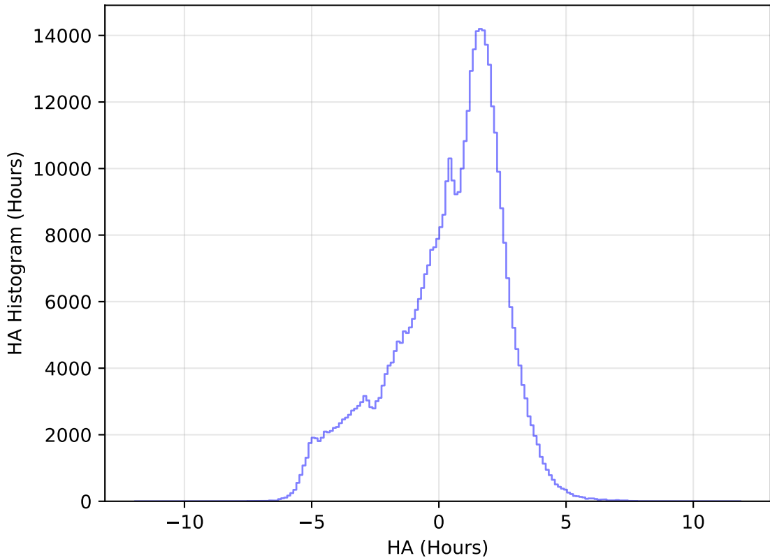
internal_u_expt60_nscale1.1v3.4_10yrs All sky r band: HA Histogram
