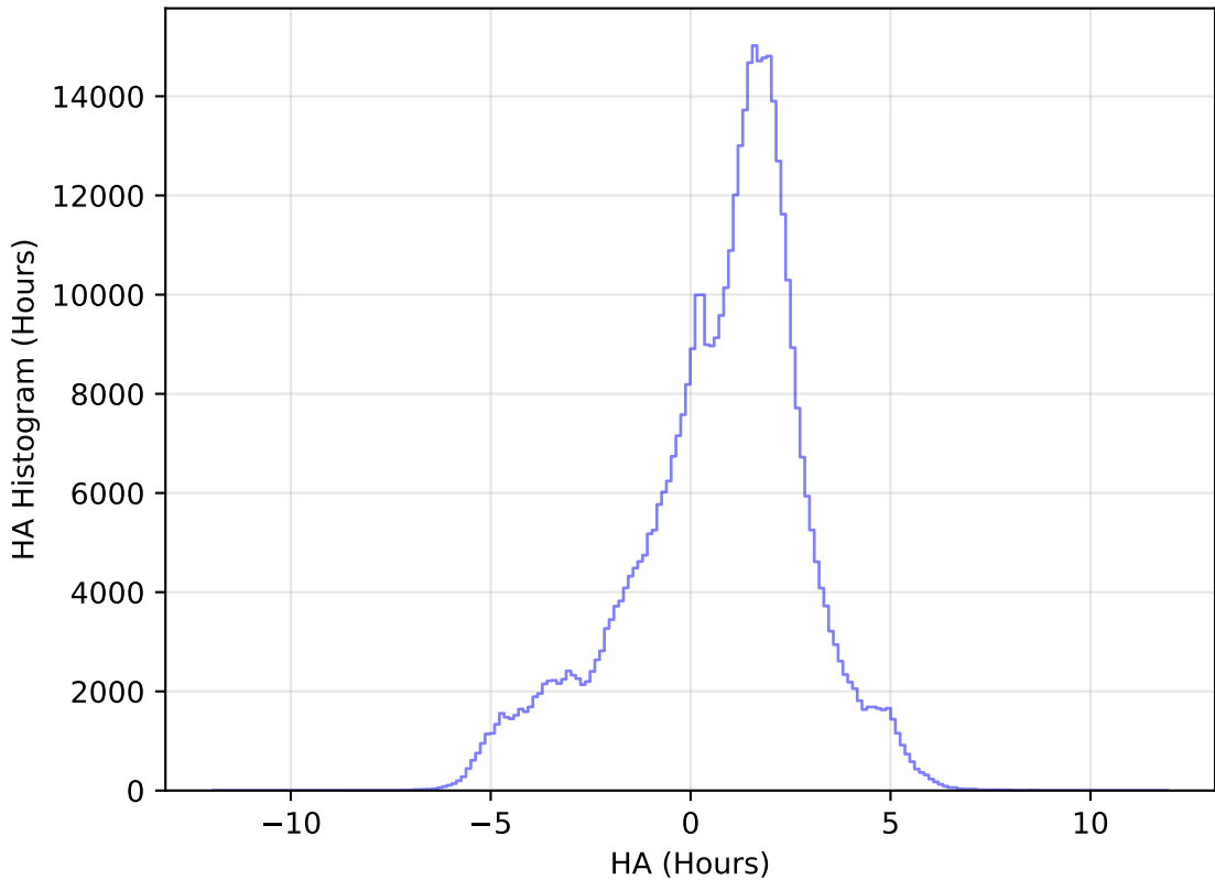
internal_u_expt60_nscale1.1v3.4_10yrs All sky i band: HA Histogram
