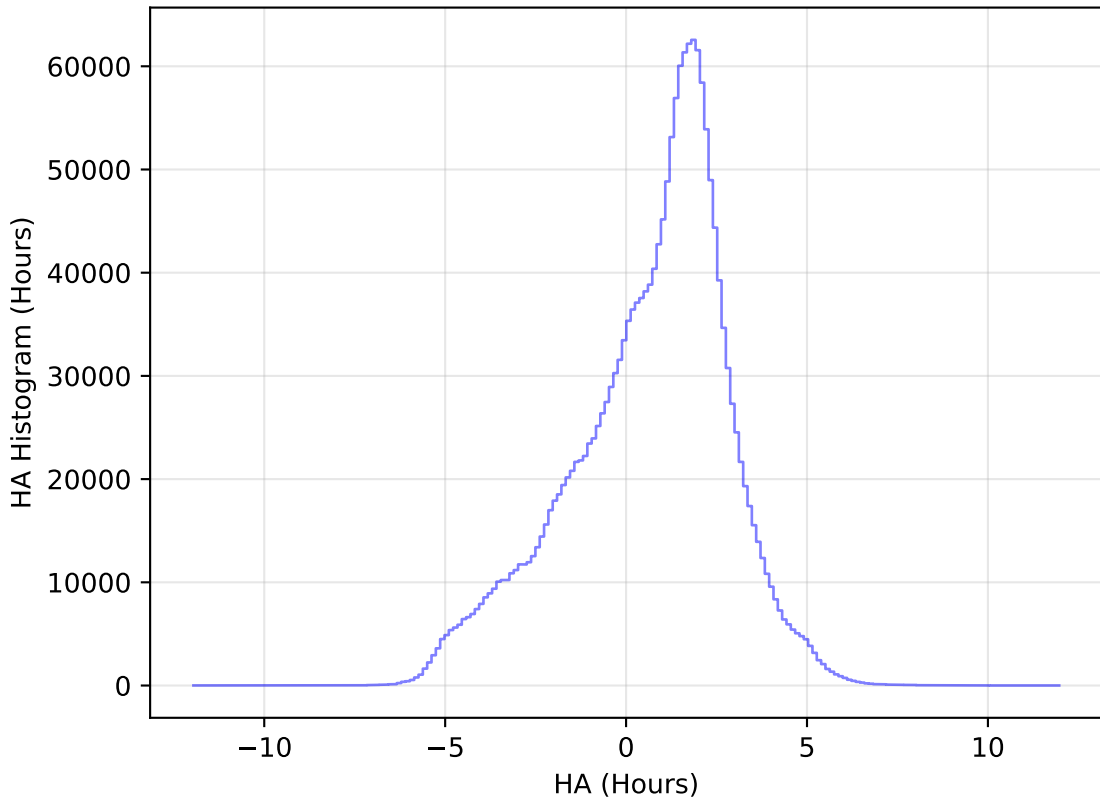
internal_u_expt60_nscale1.1v3.4_10yrs All sky all bands: HA Histogram
