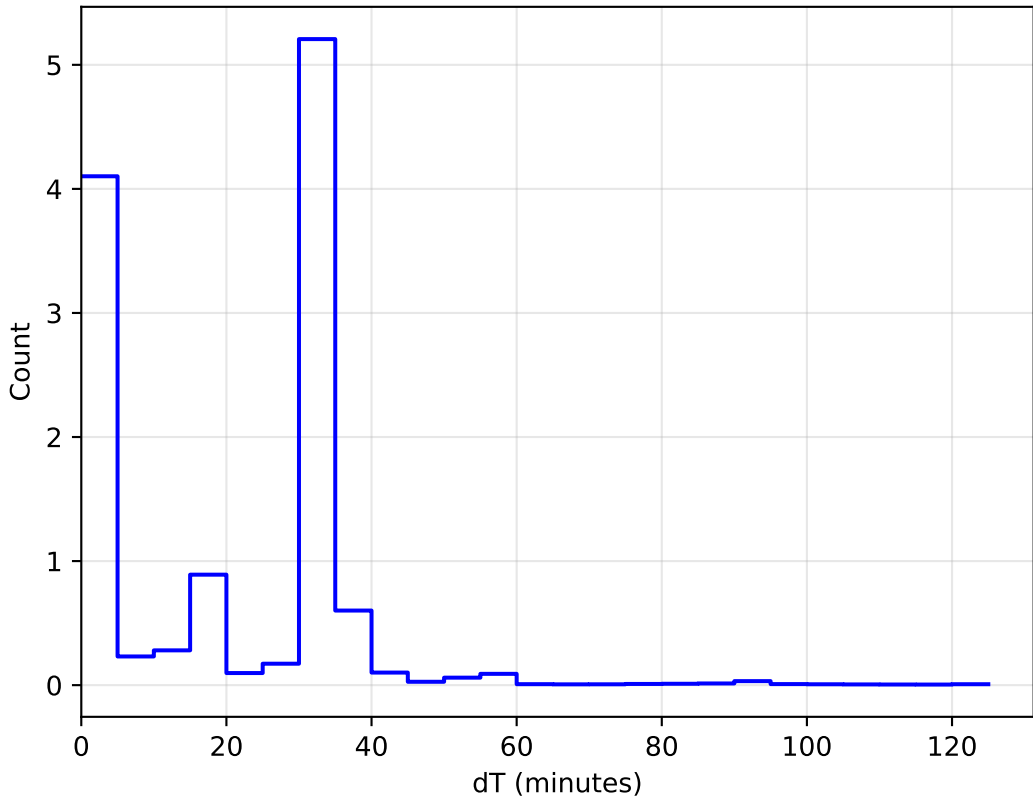
internal_u_expt60_nscale1.1v3.4_10yrs All sky: DeltaT Histogram
