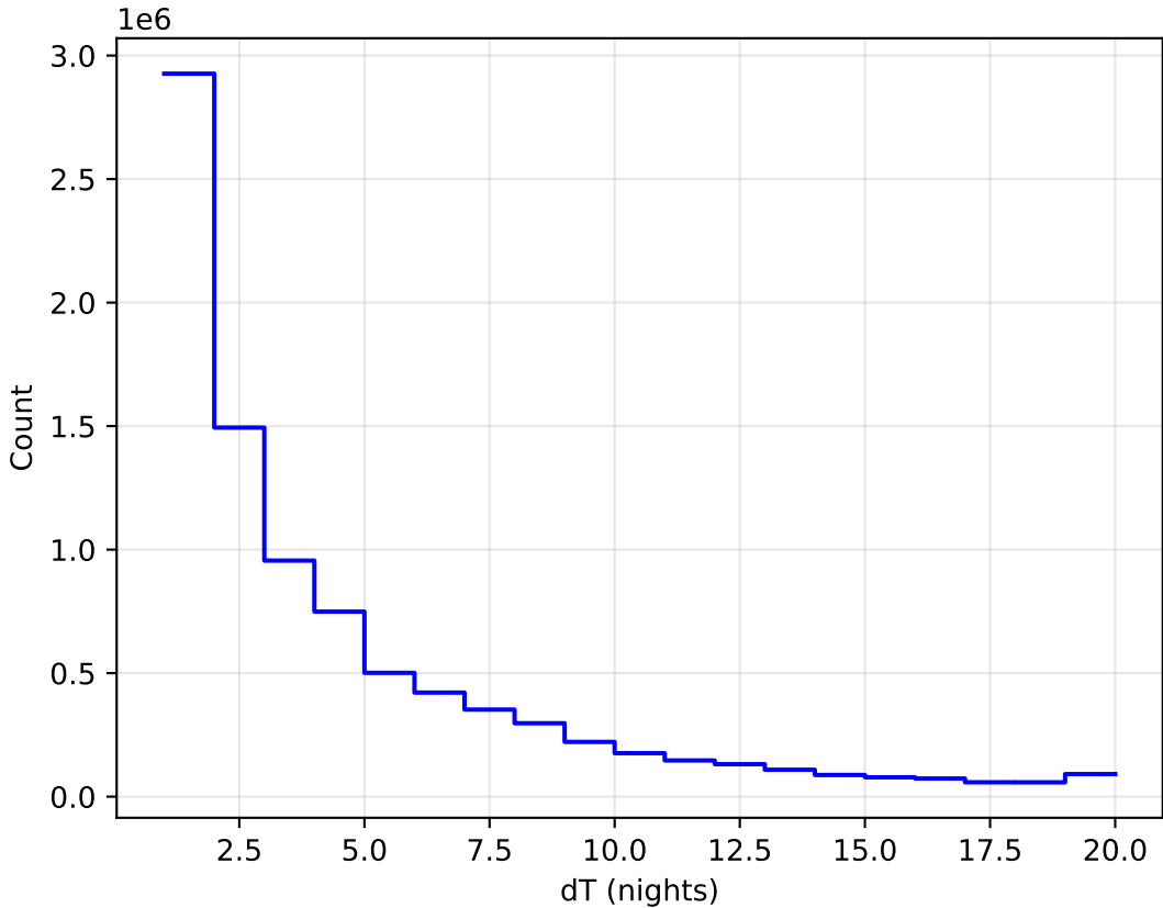
internal_u_expt60_nscale1.1v3.4_10yrs All sky all bands: DeltaNight Histogram
