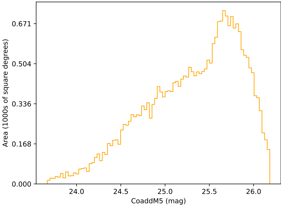
internal_u_expt60_nscale1.1v3.4_10yrs Yr 3-4 r band: CoaddM5
