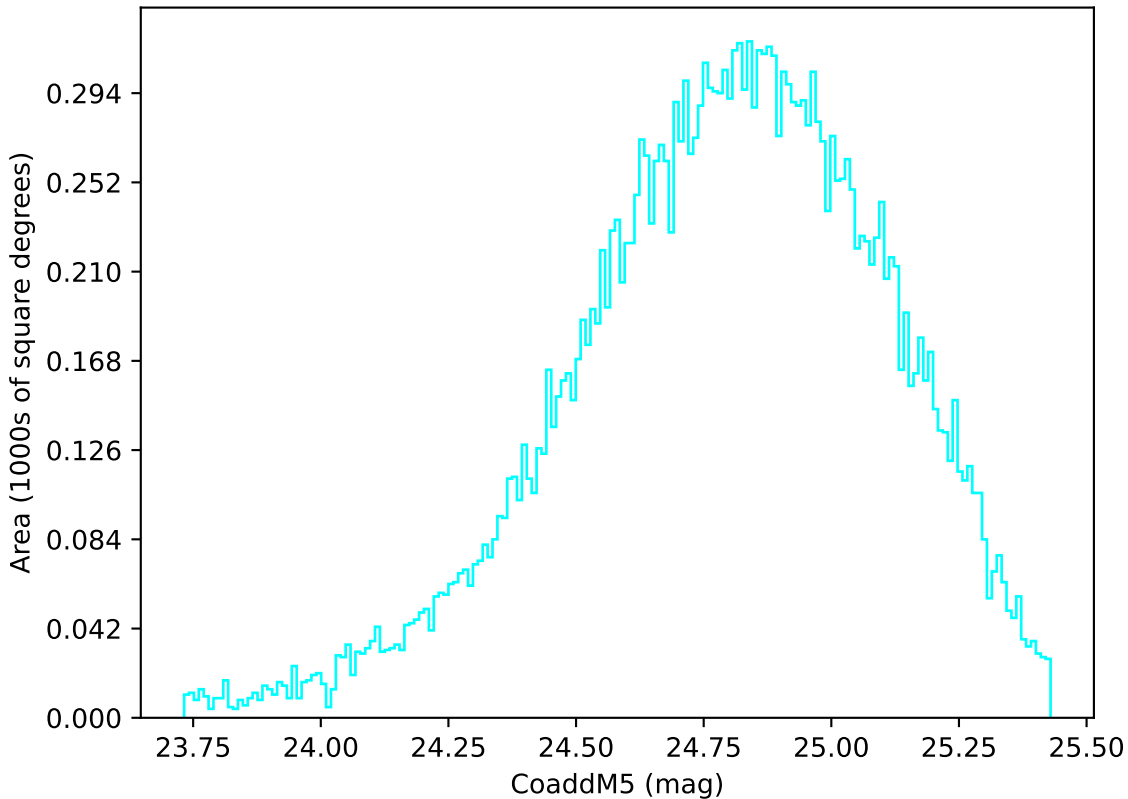
internal_u_expt60_nscale1.1v3.4_10yrs Yr 1 u band: CoaddM5
