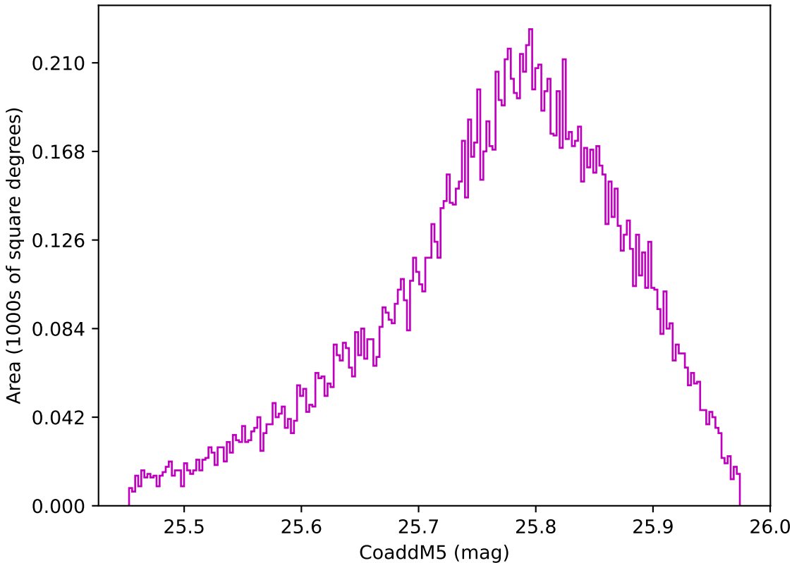
internal_u_expt60_nscale1.1v3.4_10yrs WFD z band: CoaddM5
