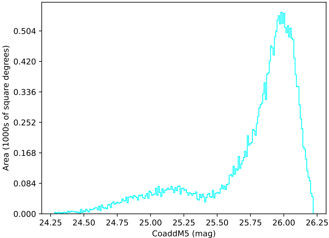
internal_u_expt60_nscale1.1v3.4_10yrs All sky u band: CoaddM5
