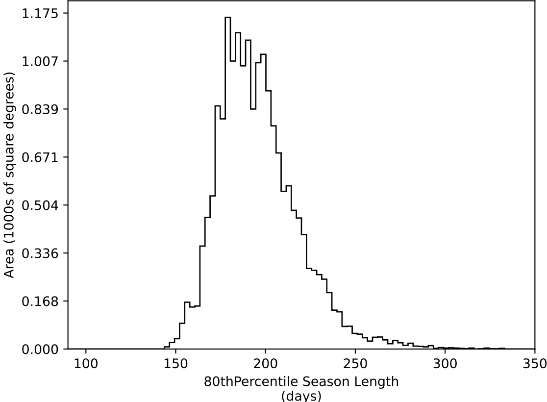
internal_u_expt60_nscale1.1v3.4_10yrs WFD all bands: 80thPercentile Season Length
