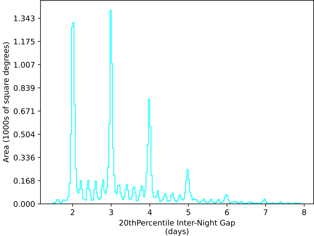
internal_u_expt60_nscale1.1v3.4_10yrs WFD u band: 20thPercentile Inter-Night Gap
