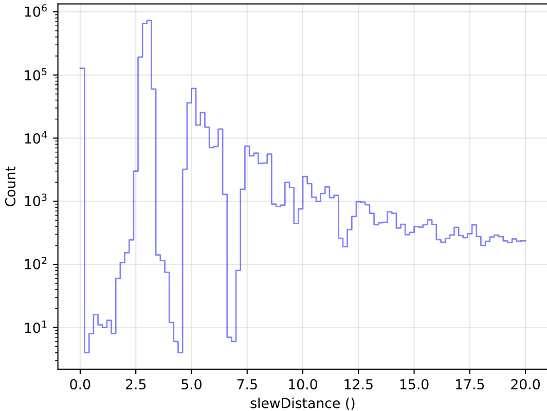
internal_u_expt60_nscale1.1v3.4_10yrs All visits: Zoom Slew Distance Histogram
