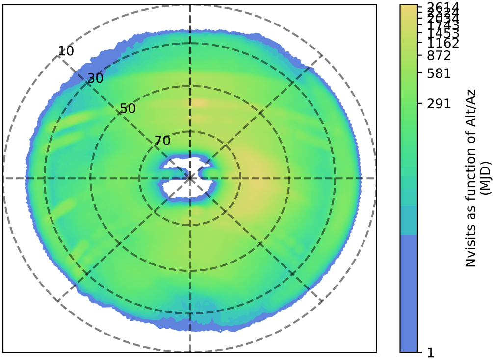
internal_u_expt60_nscale1.1v3.4_10yrs i: Nvisits as function of Alt/Az
