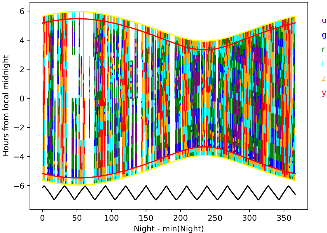
internal_u_expt60_nscale1.1v3.4_10yrs year 9-10: Hourglass
