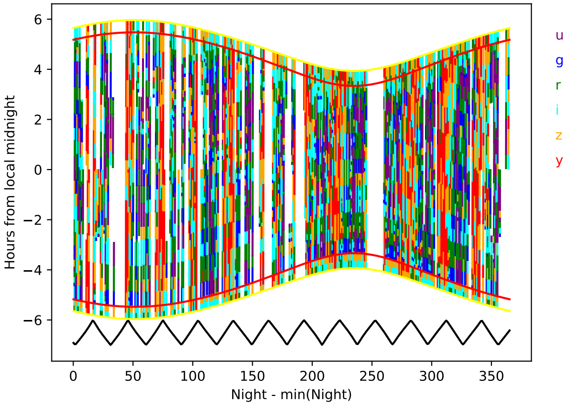
internal_u_expt60_nscale1.1v3.4_10yrs year 5-6: Hourglass
