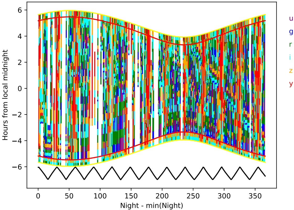
internal_u_expt60_nscale1.1v3.4_10yrs year 1-2: Hourglass
