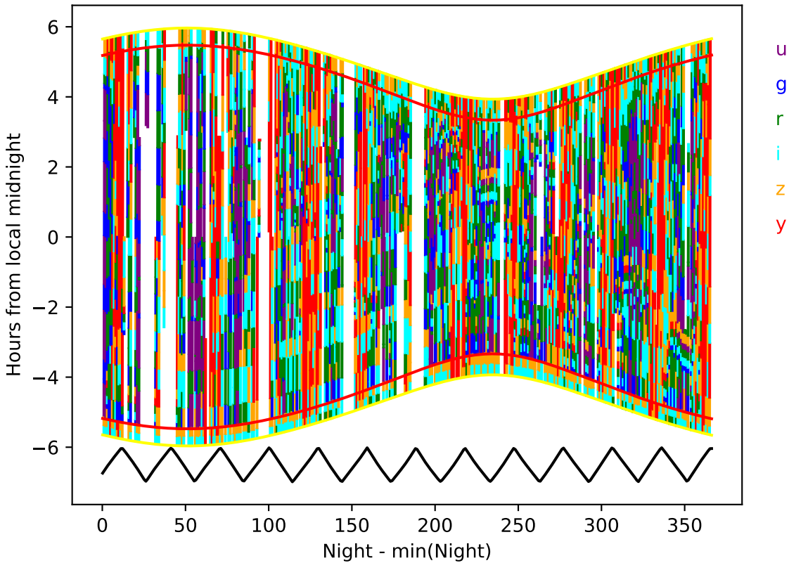
internal_u_expt60_nscale1.1v3.4_10yrs year 0-1: Hourglass
