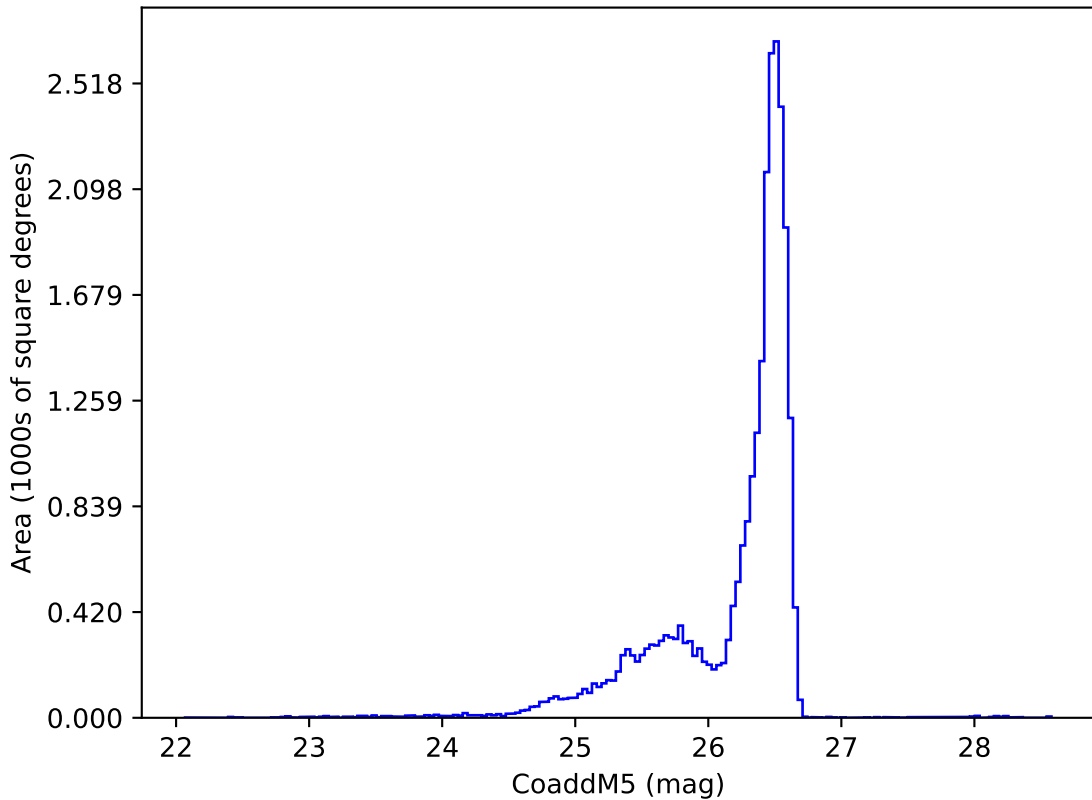
internal_u_expt60_nscale1.1v3.4_10yrs i: CoaddM5
