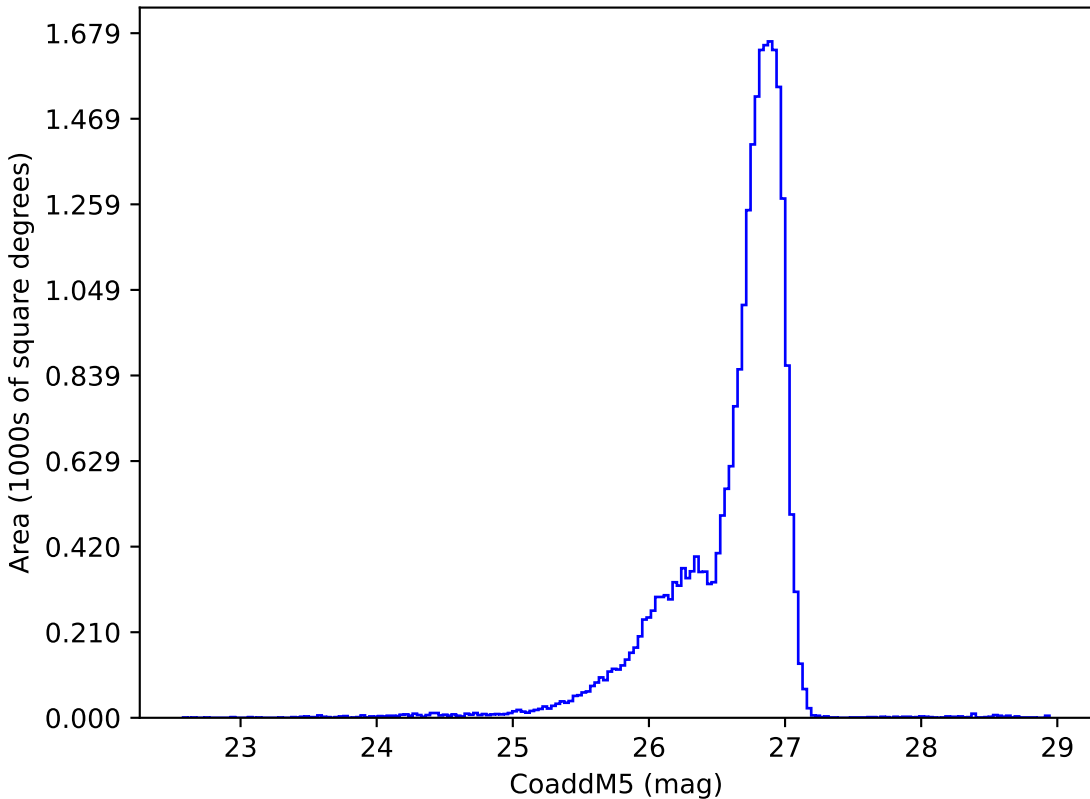
internal_u_expt60_nscale1.1v3.4_10yrs g: CoaddM5
