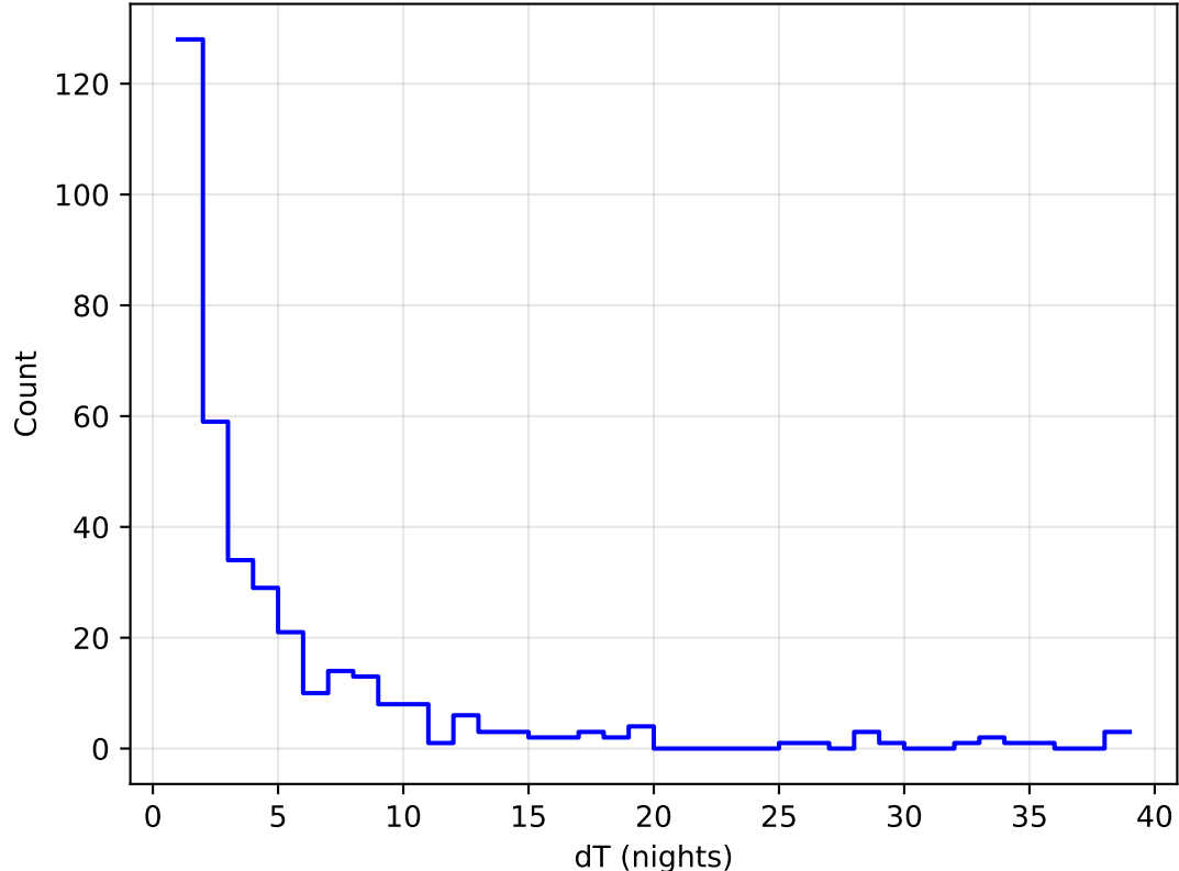
internal_u_expt60_nscale1.1v3.4_10yrs all bands: DD:WFD Delta Nights Histogram
