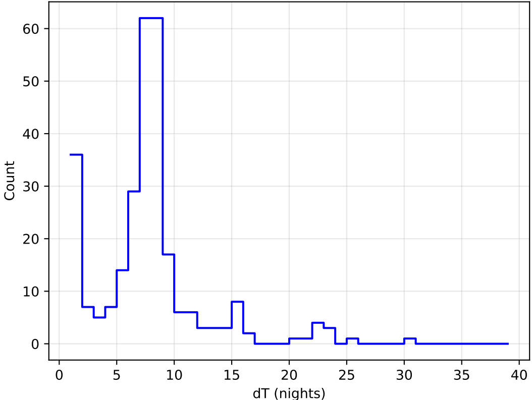
internal_u_expt60_nscale1.1v3.4_10yrs all bands: DD:ECDFS Delta Nights Histogram
