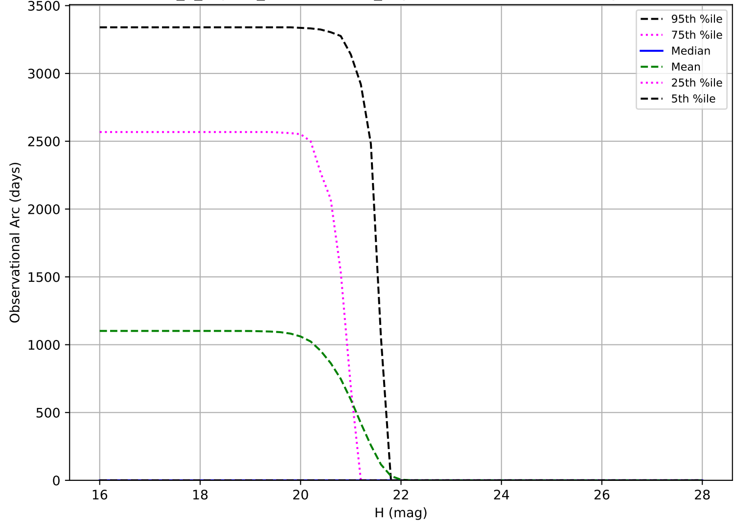
internal_u_expt60_nscale1.0v3.4_10yrs: Observational Arc Length Vatra
