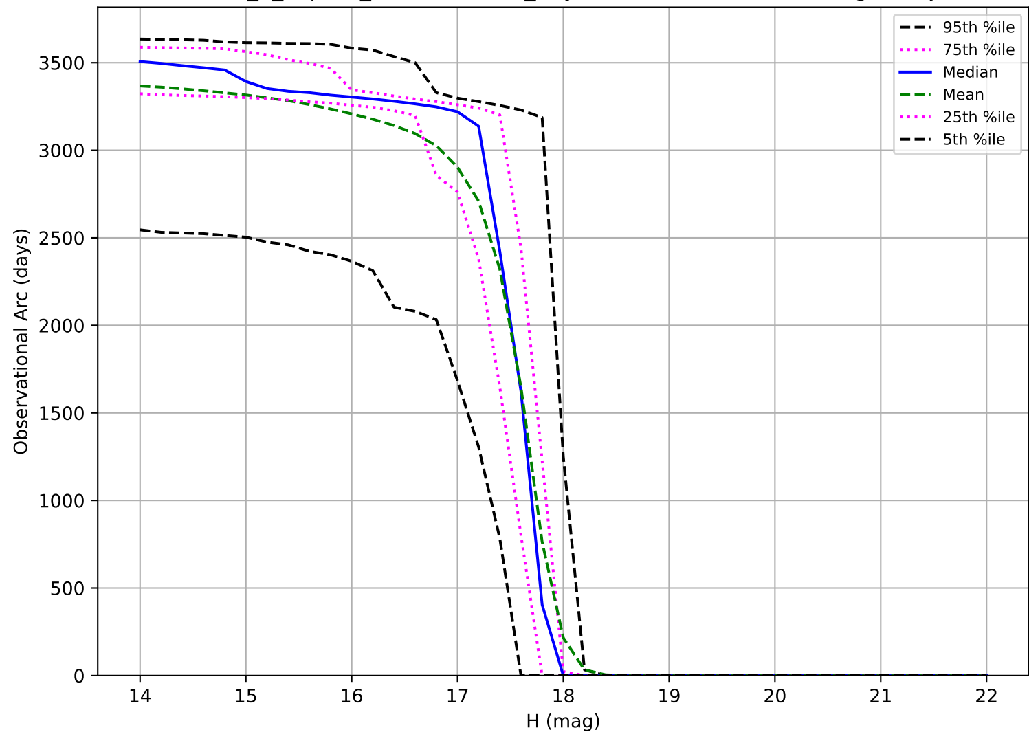
internal_u_expt60_nscale1.0v3.4_10yrs: Observational Arc Length Trojan
