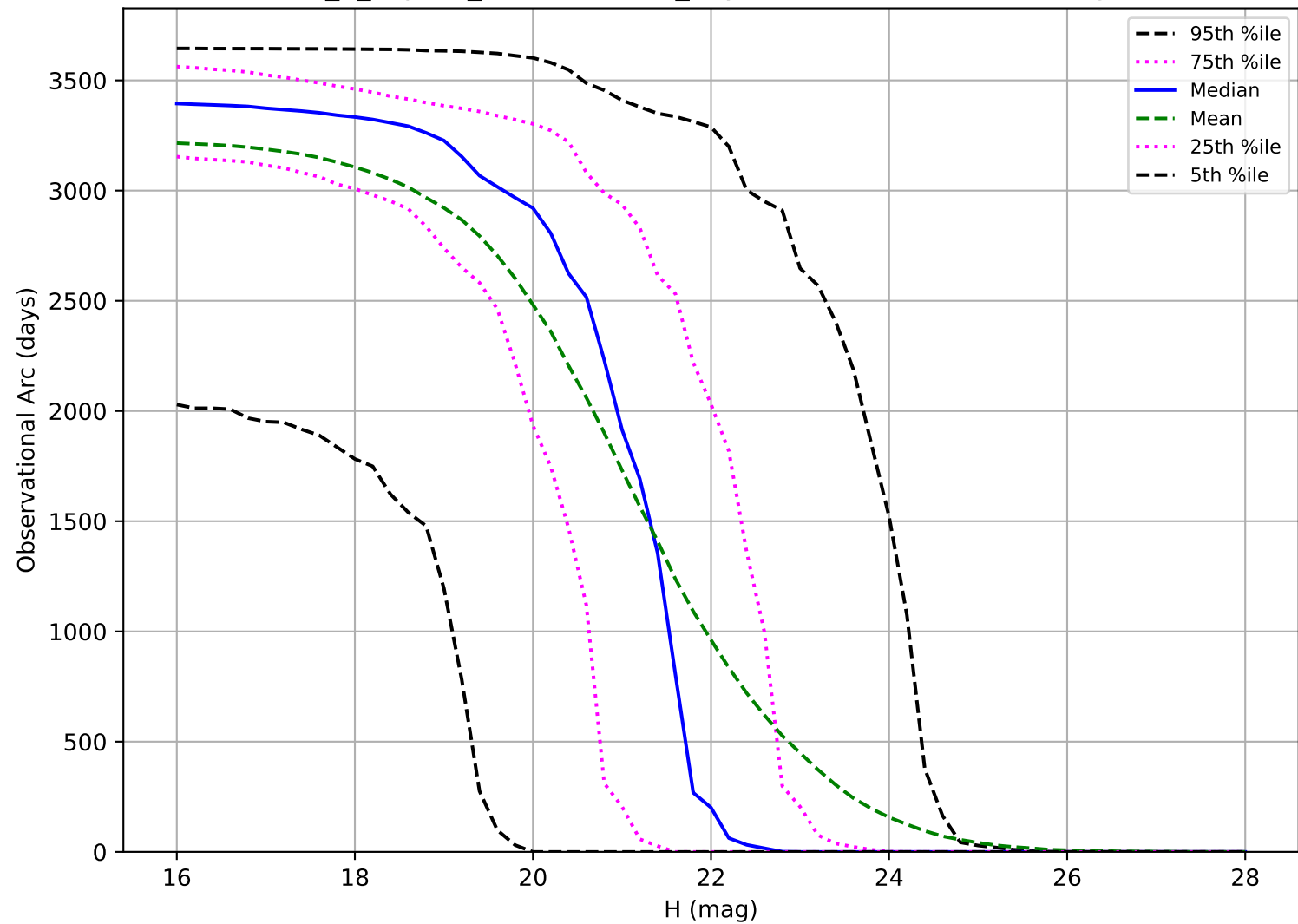
internal_u_expt60_nscale1.0v3.4_10yrs: Observational Arc Length PHA
