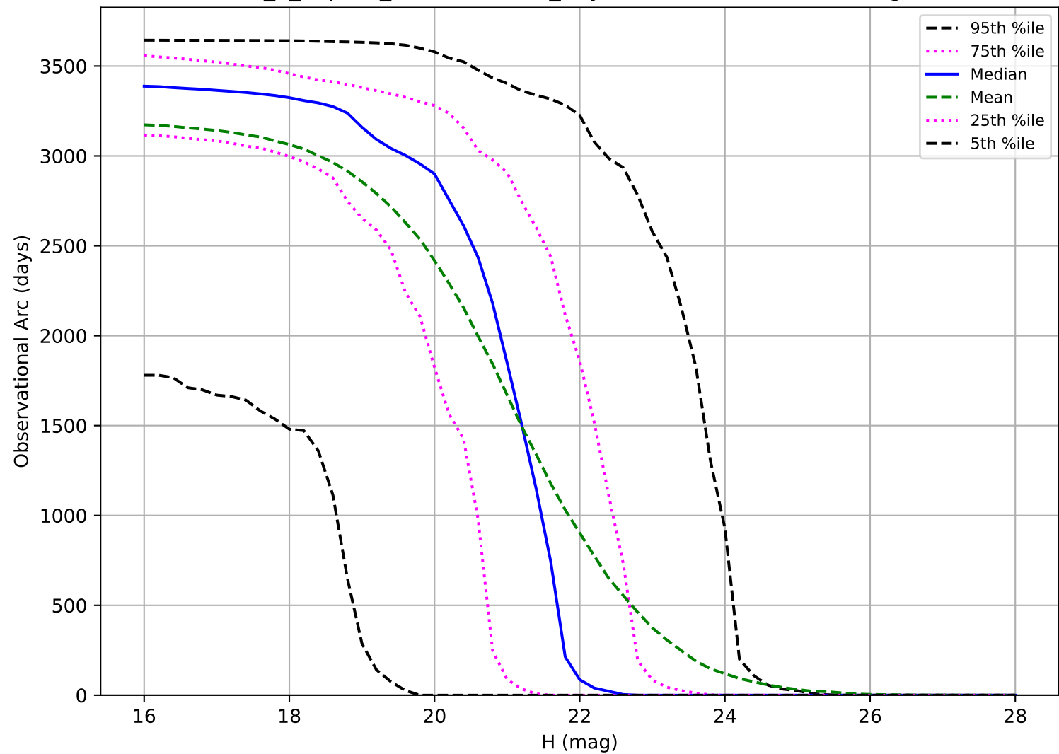
internal_u_expt60_nscale1.0v3.4_10yrs: Observational Arc Length NEO
