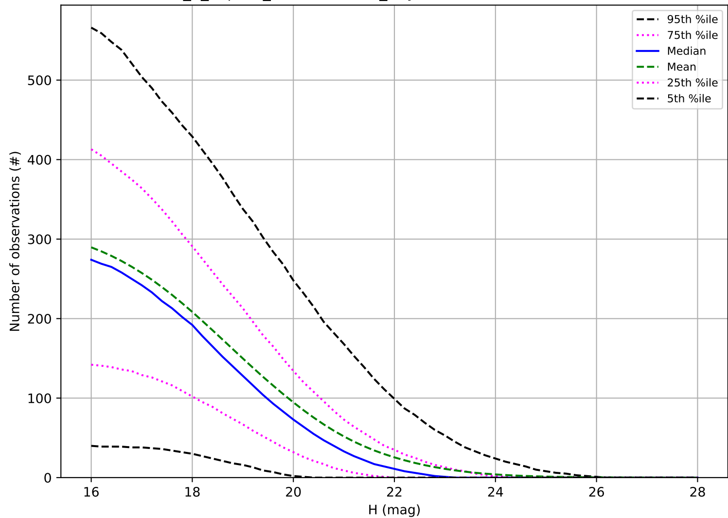
internal_u_expt60_nscale1.0v3.4_10yrs: Number of observations PHA
