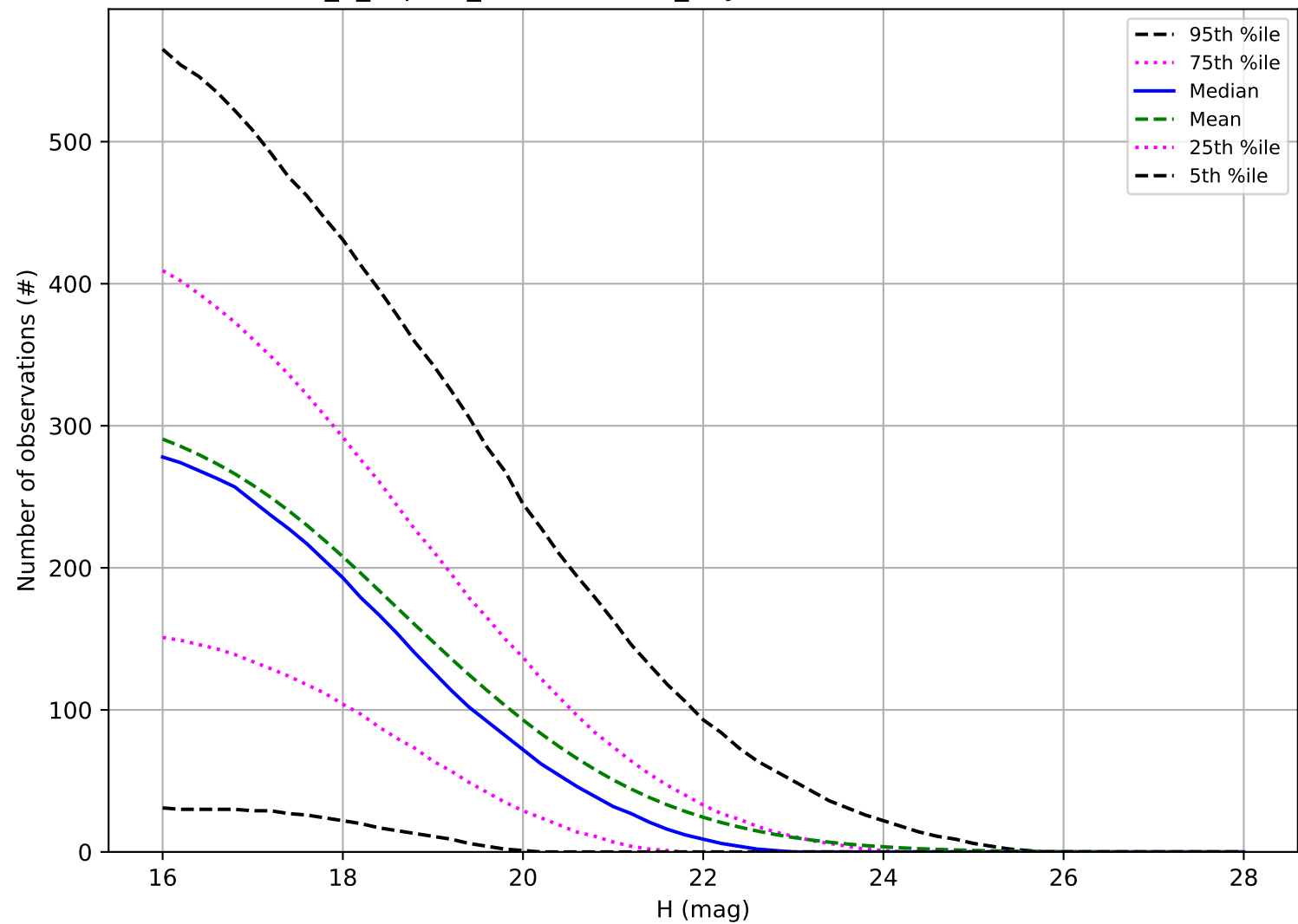
internal_u_expt60_nscale1.0v3.4_10yrs: Number of observations NEO
