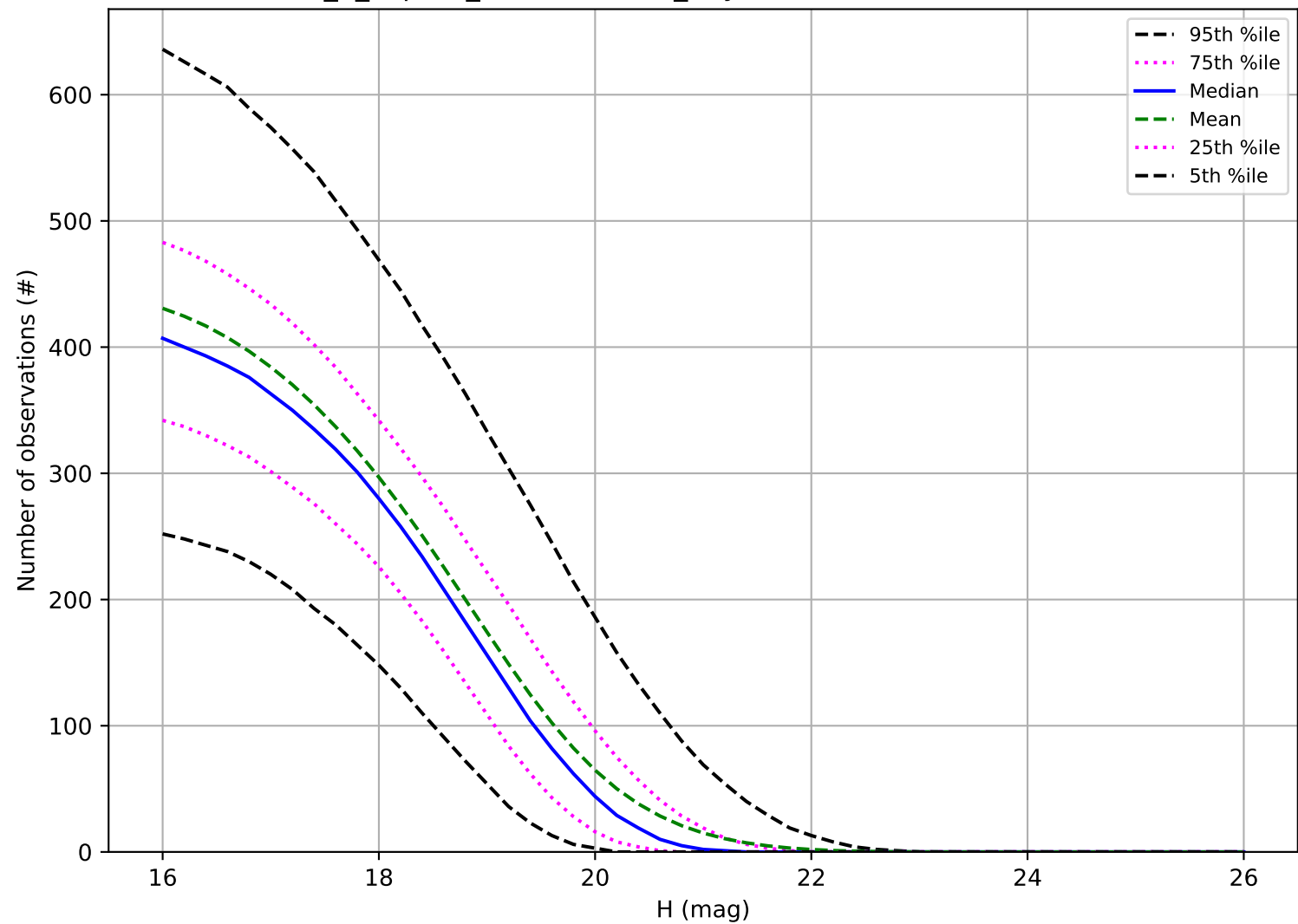
internal_u_expt60_nscale1.0v3.4_10yrs: Number of observations MBA
