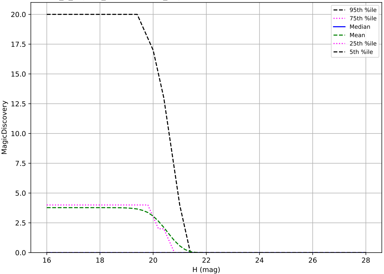
internal_u_expt60_nscale1.0v3.4_10yrs: Vatira 6 detections in 60 nights detection loss
