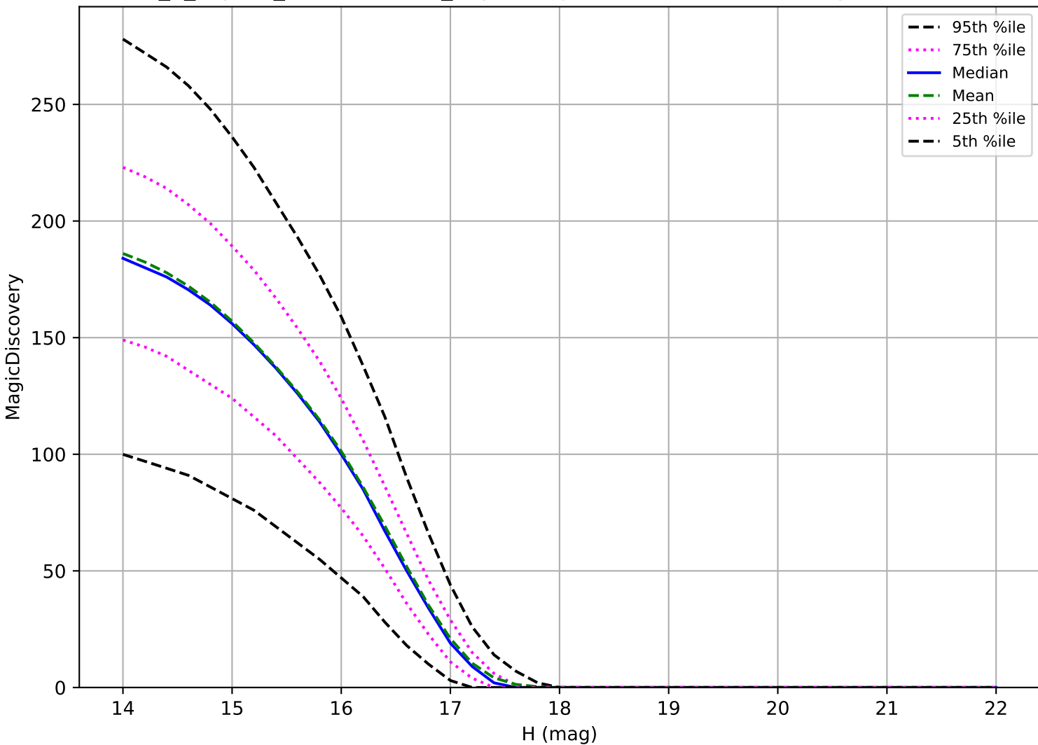
internal_u_expt60_nscale1.0v3.4_10yrs: Trojan 6 detections in 60 nights detection loss
