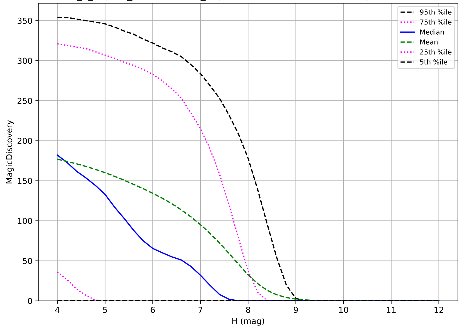
internal_u_expt60_nscale1.0v3.4_10yrs: TNO 6 detections in 60 nights detection loss
