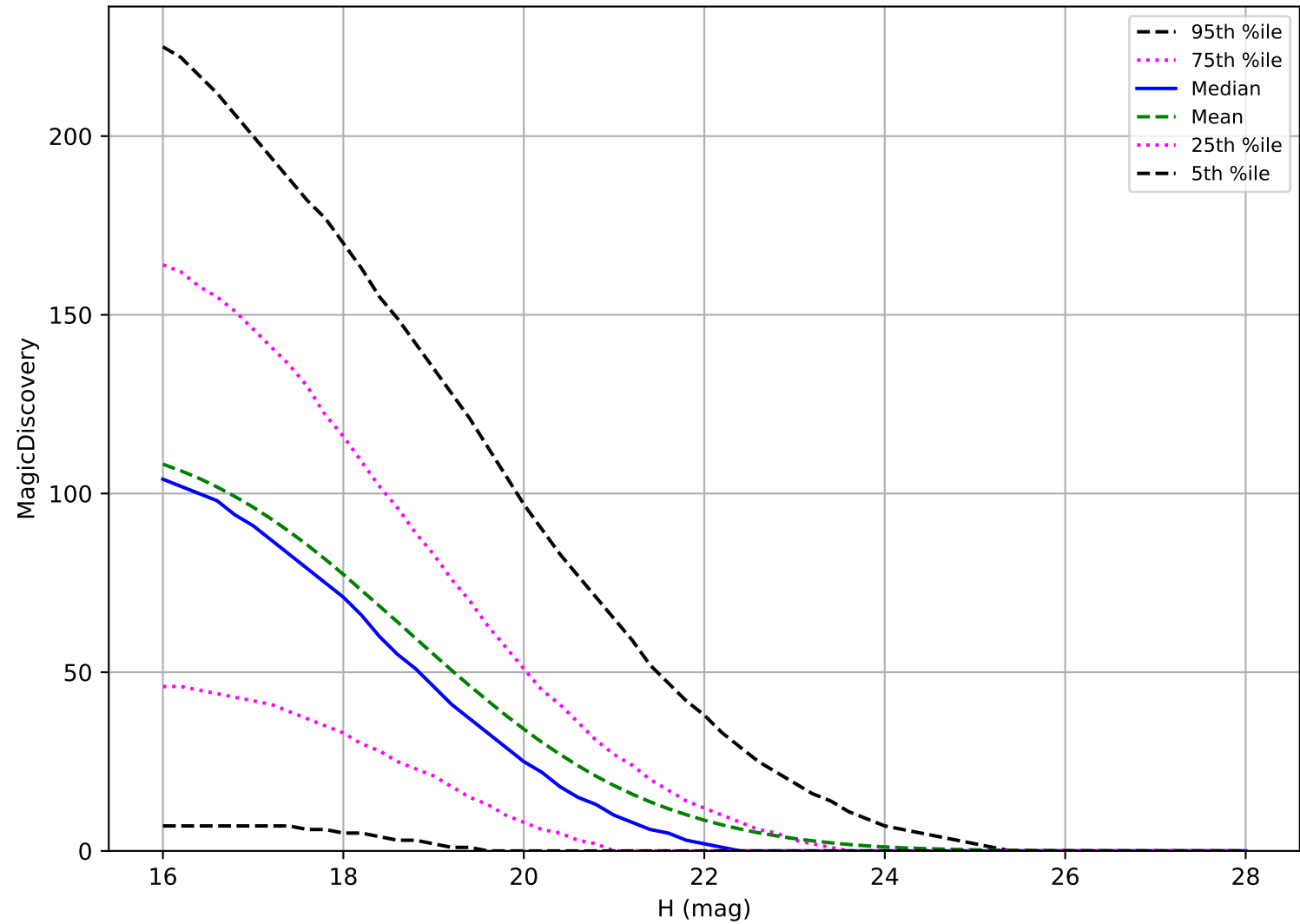
internal_u_expt60_nscale1.0v3.4_10yrs: PHA 6 detections in 60 nights detection loss
