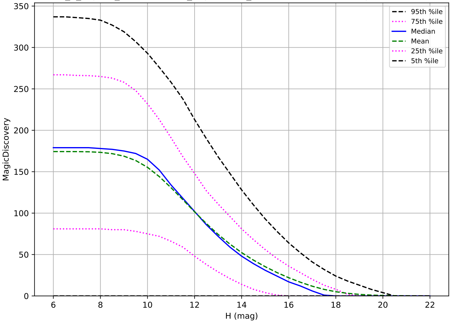
internal_u_expt60_nscale1.0v3.4_10yrs: OCC_r5 6 detections in 60 nights detection loss
