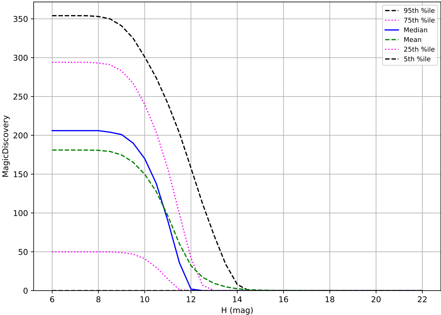
internal_u_expt60_nscale1.0v3.4_10yrs: OCC_r20 6 detections in 60 nights detection loss
