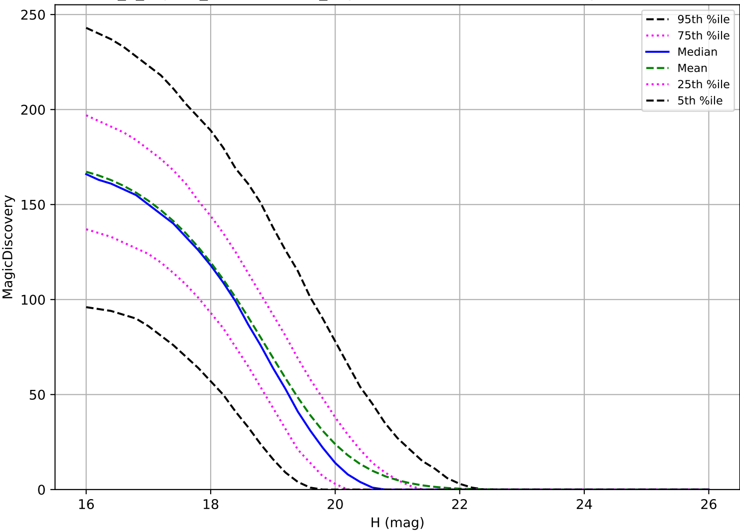
internal_u_expt60_nscale1.0v3.4_10yrs: MBA 6 detections in 60 nights detection loss
